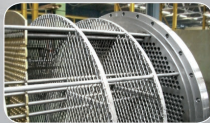
"Hybrid" EMbaffle® Anti-vibration Solution for conventional baffled heat exchangers
