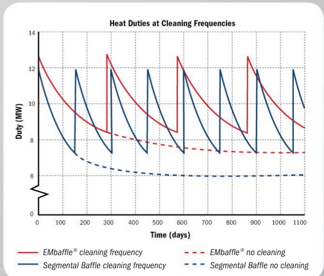
Increased run time for the EMbaffle® heat exchanger
